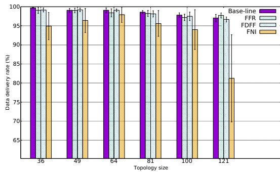
Figure 5: Data packet delivery rates for one attacker
